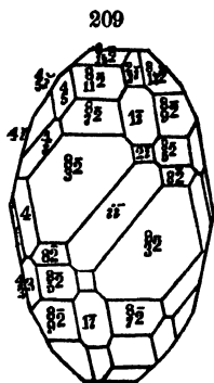
Humite.
